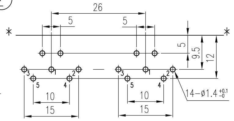
P.C.B Layout Dimension (Tolerance:±0.1) (Recommend min.Dimension)(bottom view)
