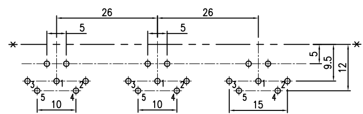
P.C.B Layout Dimension(Tolerance:±0.1) (Recommend min. Dimension)(Bottom View)
