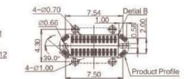
RECOMMENDED P.C.B LAYOUT (COMPONENT SIDE) PCB THICKNESS: 1.20 \pm 0.05 mm DEFAULT TOLERANCE: \pm 0.05
