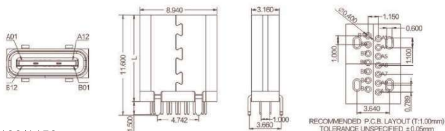
TYPE-C 14P-F 立式直插DIP鱼叉脚 H=9.3/10.0/10.5/11.50mm
