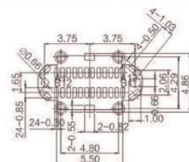
RECOMMENDED PCB LAYOUT PCB T=1.20mm TOL: \pm 0.05
