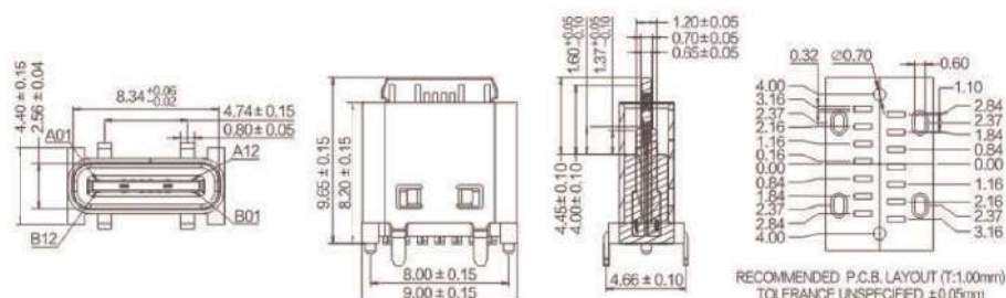
TYPE-C 14P-F 立式贴片SMT H=9.3/10.0/10.50mm
