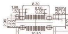
RECOMMENDED PCB LAYOUT TOL: \pm 0.05
