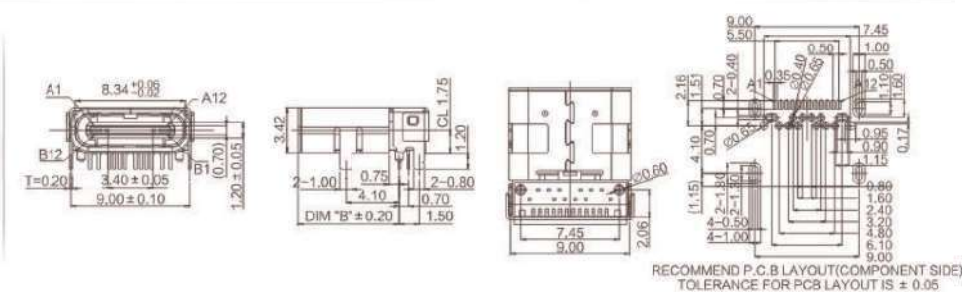
TYPE-C 24P-F 板上四脚插板DIP+SMT双壳 L=8.65/10.0mm
