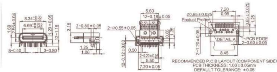
TYPE-C 24P-F 板上四脚插板DIP+SMT L=8.59mm
