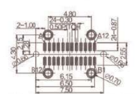
RECOMMENDED P.C.B LAYOUT (T:1.00mm) TOLERANCE UNSPECIFIED \pm 0.05 mm
