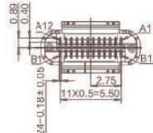
RECOMMENDED P.C.B LAYOUT (COMPONENT SIDE) PCB THICKNESS: 1.20 \pm 0.05 mm DEFAULT TOLERANCE: \pm 0.05
