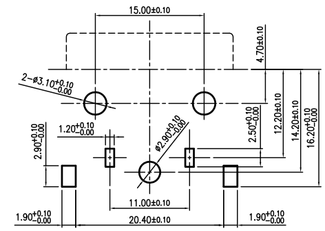
PCB Layout Dimension (Tolerance:±0.10) (Recommend min. Dimension)(Bottom View) Scale 2:1
